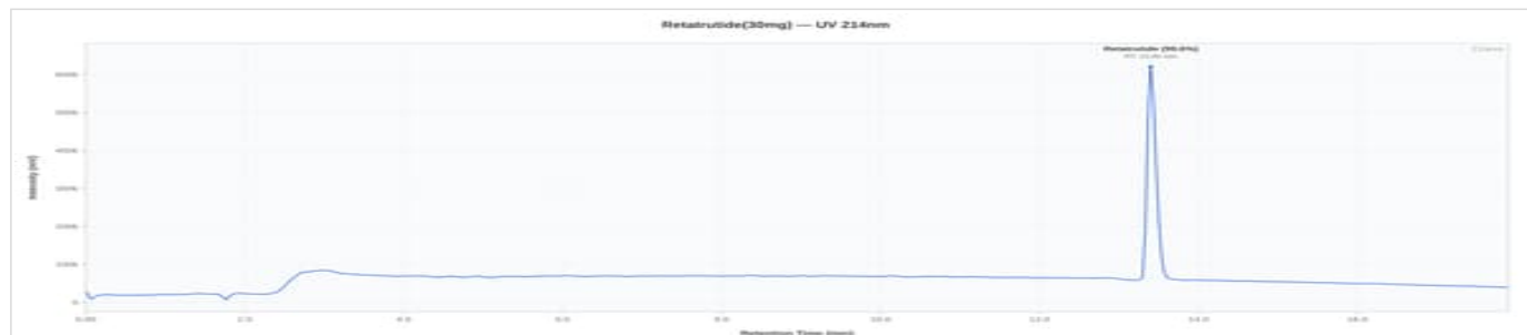
Retatrutide 30mg - RRL-RT30-001-0726: UV Chromatogram
